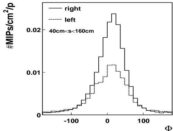
Fig.4: Angular distribution of MIPs outside the vacuum vessel for impact of proton on the right side of the beam screen, and on the left side
