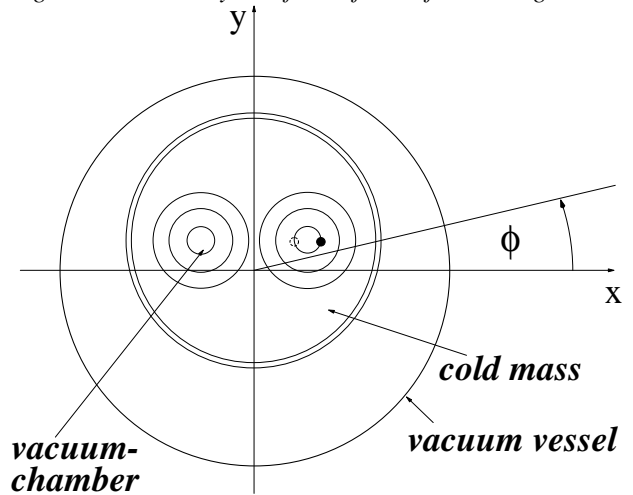
Fig.1: Schematic layout of a half cell of 53 m length
