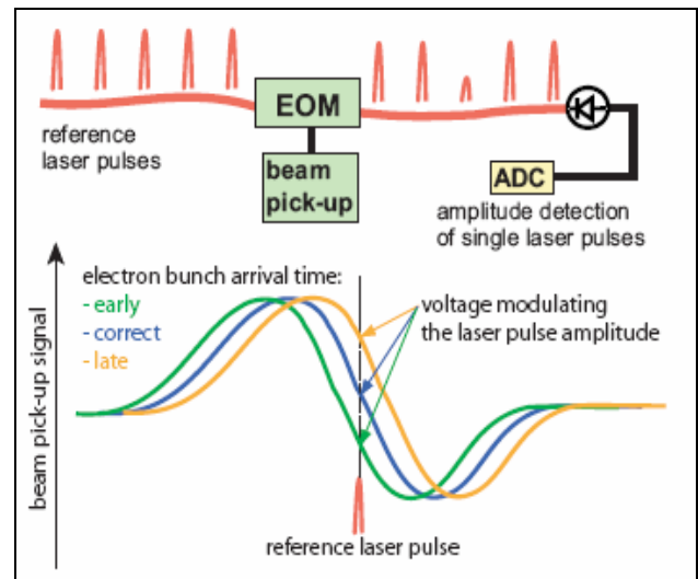
Fig. 1: Principle of the arrival time detection (from Ref. 15)
