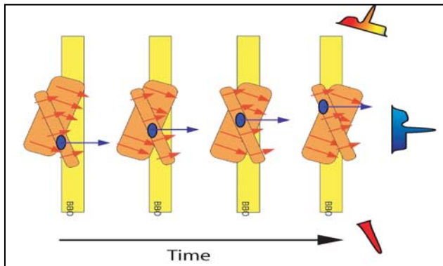
Fig. 8: Schematic of the single shot cross correlator (BBO) (from Ref. 26)
