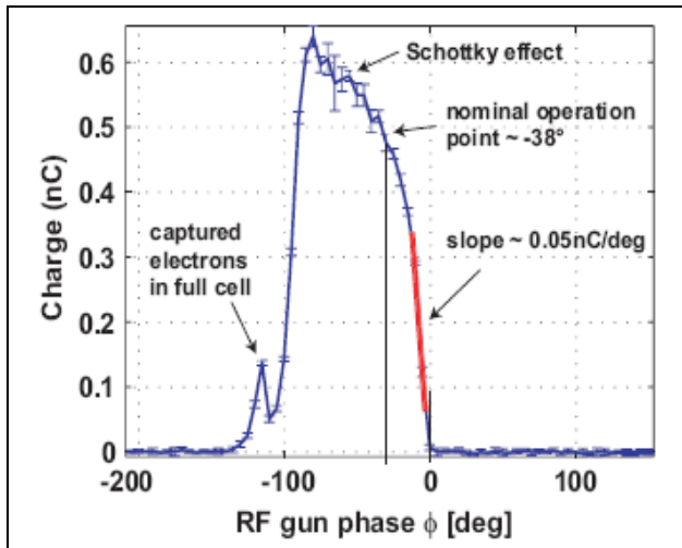
Fig. 4: Beam current versus gun phase (from Ref. 17)
