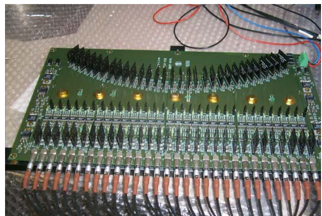
Fig. 5: Photo of the 30 channel pyro-line-detector of the single shot spectrometer (from Ref. 21).
