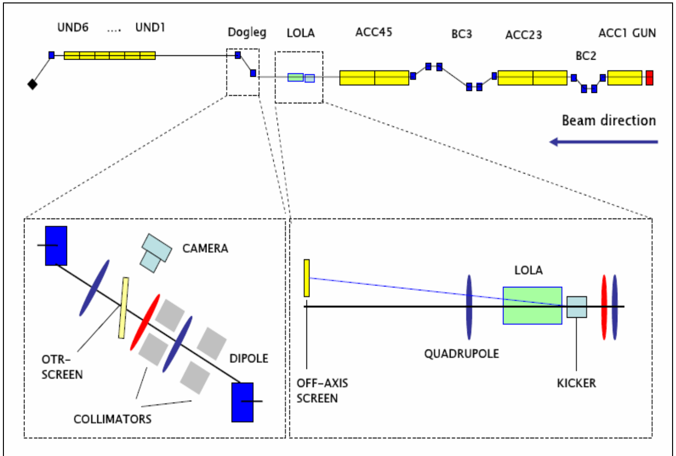
Fig. 6 bottom left: Slice energy spread measurement in a dispersive section of FLASH, Fig. 5 bottom right: Longitudinal profile and slice emittance measurement with an off-axis screen. Fig. 5 top: Schematic of the FLASH beam line (from Ref. 23).
