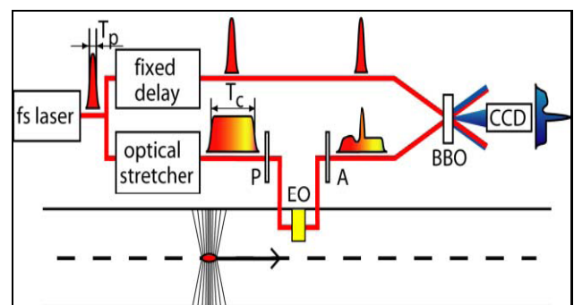
Fig. 7: Schematic setup of the single shot bunch length measurement technique using electro optical sampling (from Ref. 24).
