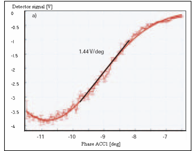
Fig. 3: Phase scan of acceleration module (from Ref. 17).
