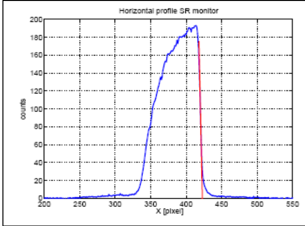
Fig. 2: Horizontal beam profile from the synchrotron monitor in the first magnetic chicane (from Ref. 17).
