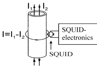
Figure 1: Scheme of a SQUID-based CCC.
