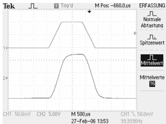
Figure 4: Current pulse test signal (upper curve) and SQUID output signal (lower curve).
