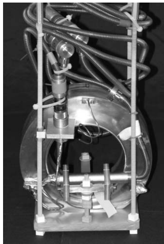
Figure 3: Nb pick-up coil prepared for tests at 4.2 K.
