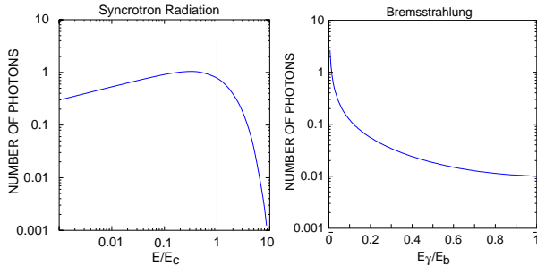
Figure 2: Photon spectrum from synchrotron radiation and bremsstrahlung.
